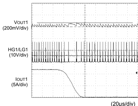
Fig.11 Vout1 transient response
