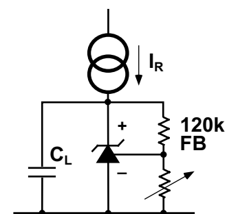
* Output Impedance vs. Freq. Test Circuit
