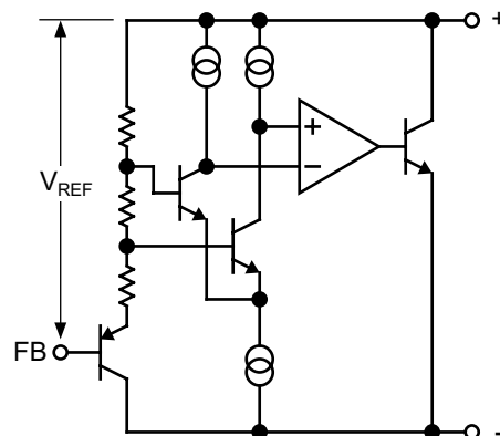
Functional Diagram LM4041 Adjustable
