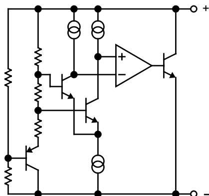
Functional Diagram LM4040, LM4041 Fixed
