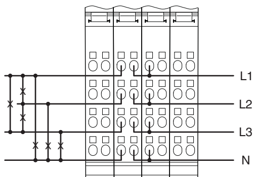
Figure 4 Direct connection
