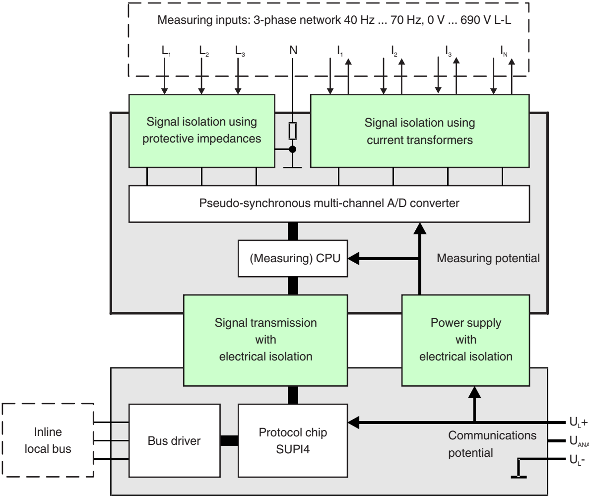
Figure 1 Internal basic circuit diagram
