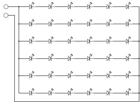
Figure 5: Electrical circuit diagram for L235-xyyyAHLGBAAC0.
