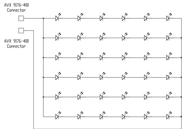
Figure 11: Electrical circuit diagram for L235-xyyyAHLCBAC0.
