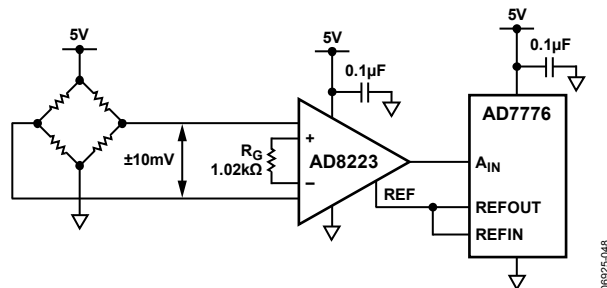
Figure 41. A Single-Supply Data Acquisition System
