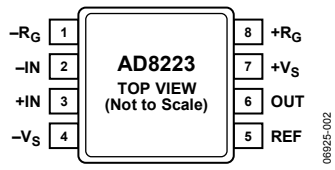
Figure 2. Pin Configuration
