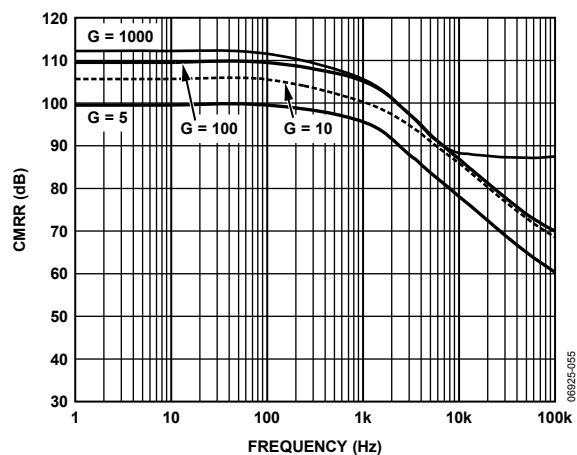
Figure 12. CMRR vs. Frequency, \pm V_S = \pm 12 V
