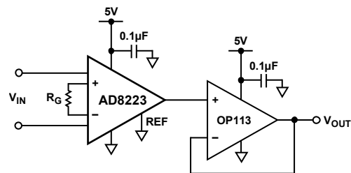
Figure 38. Output Buffering
