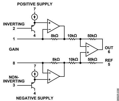
Figure 31. Simplified Schematic
