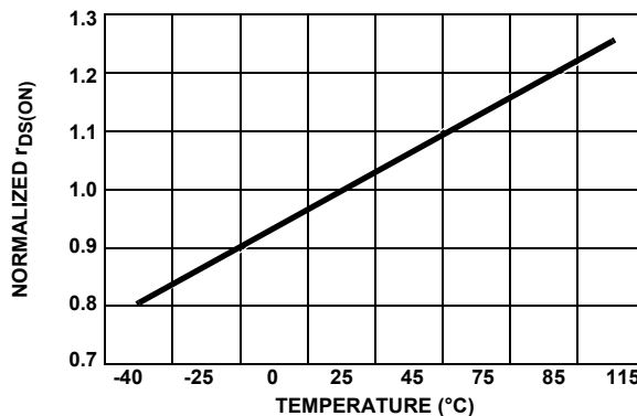
FIGURE 2. NORMALIZED r DS(ON) TEMPERATURE CHARACTERISTIC CURVE
