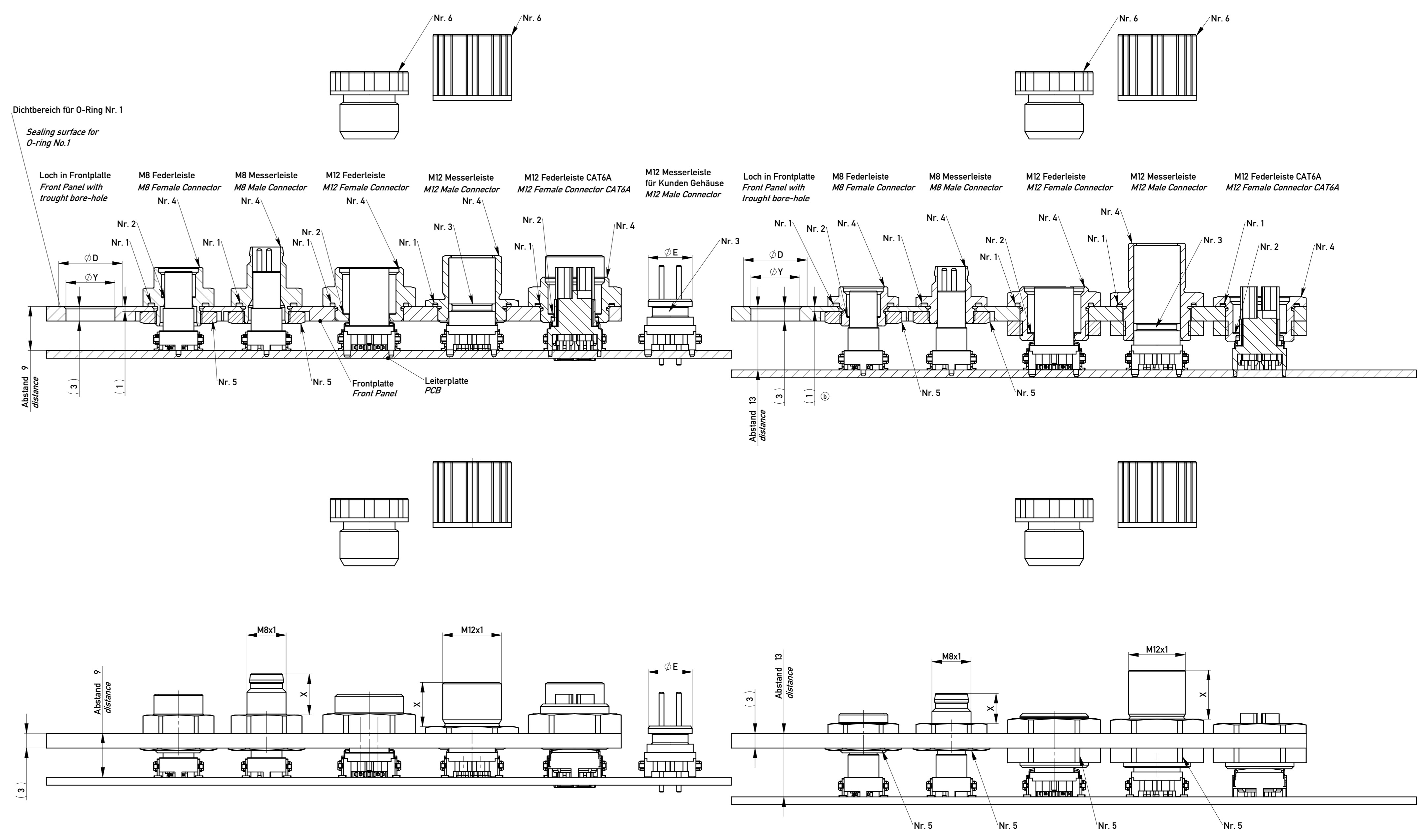
Abstand 9 mm PCB to Frontpanel distance 9mm
