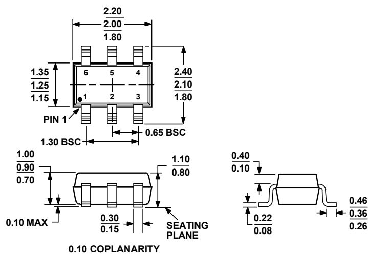
COMPLIANT TO JEDEC STANDARDS MO-203-AB Figure 59. 6-Lead Thin Shrink Small Outline Transistor Package [SC-70] (KS-6) Dimensions shown in millimeters
