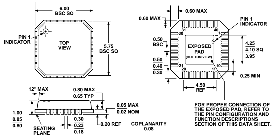
Figure 57. 40-Lead Lead Frame Chip Scale Package [LFCSP_VQ] 6 mm \times 6 mm Body, Very Thin Quad (CP-40-1) Dimensions shown in millimeters
