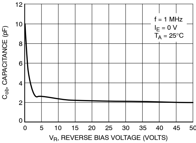
Figure 73. Output Capacitance
