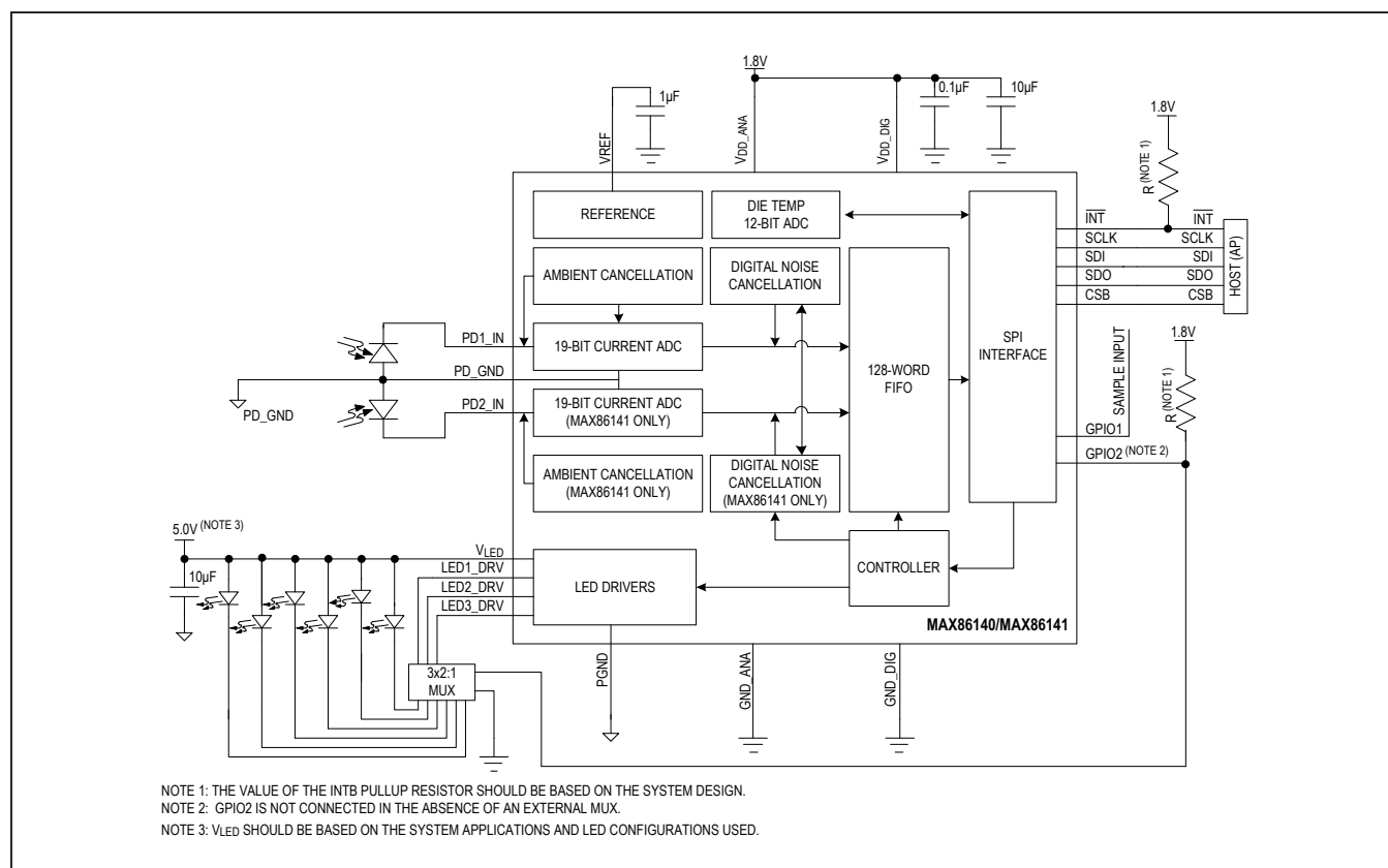
Figure 10. Block Diagram for GPIO CTRL[3:0] 0010 Without External Mux
