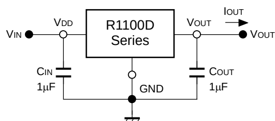
Standard Test Circuit
