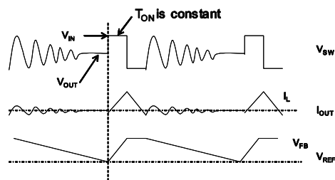
Figure 3—Light Load Operation
