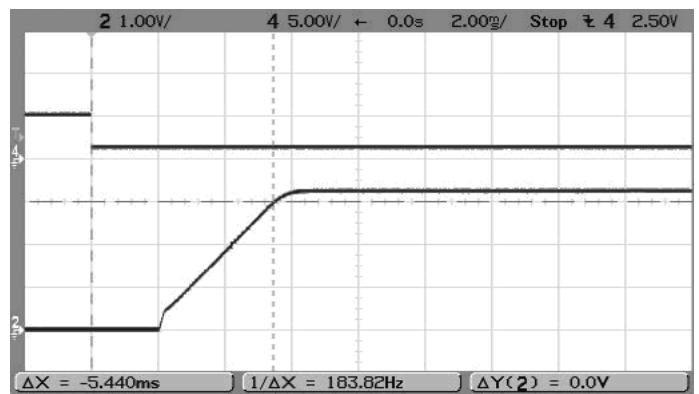
On/Off Enable Startup (V in =5V, V out =3.3V, I out =6A, Cload=0) Trace 4=Enable, Trace 2=V out
