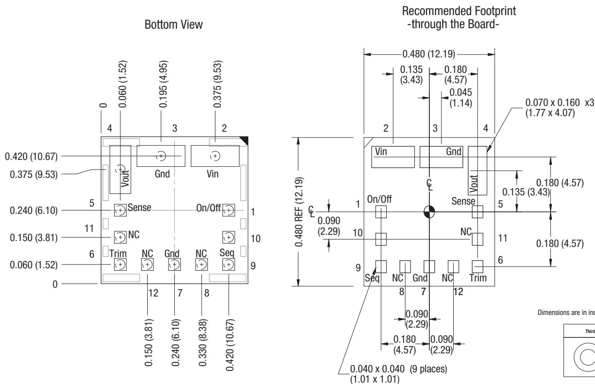
Figure 3. OKL-T/6-W5 Mechanical Outline
