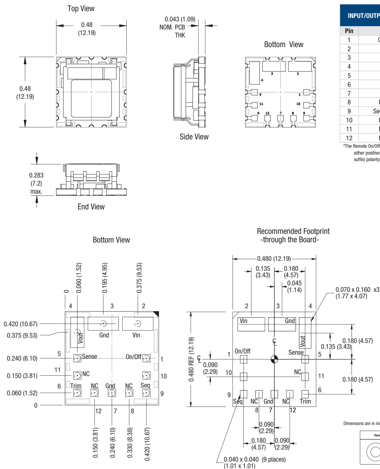
Figure 3. OKL-T/6-W5 Mechanical Outline
