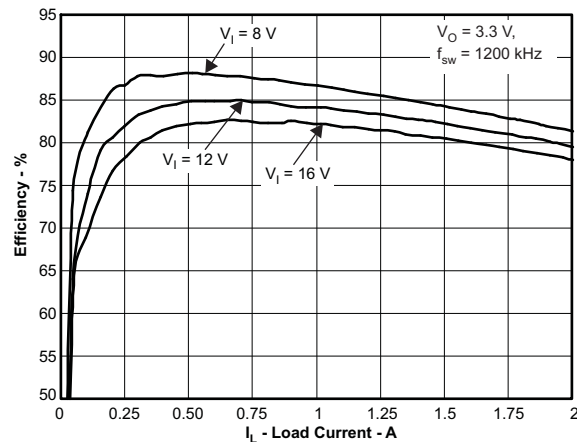
Figure 60. Efficiency vs Load Current
