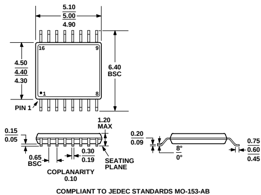
Figure 63. 16-Lead Thin Shrink Small Outline Package [TSSOP] (RU-16)
