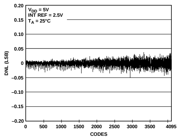
Figure 18. DNL AD5628-2
