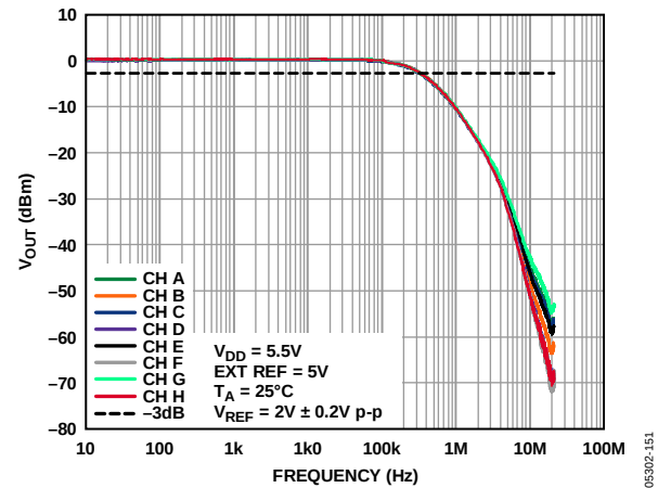
Figure 52. Multiplying Bandwidth
