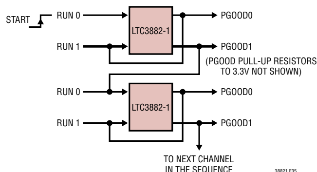
Figure 35. Cascade Sequencing Configuration
