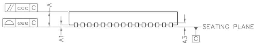
SIDE VIEW
