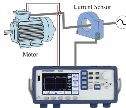
Power Meter
