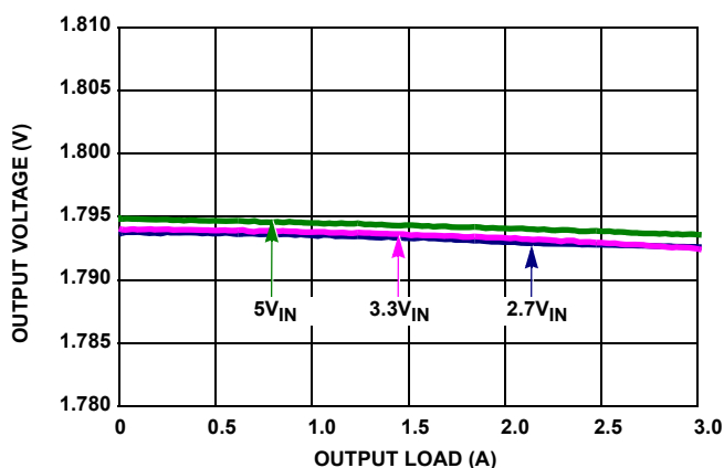
FIGURE 34. V_{OUT} REGULATION vs LOAD, 1.8V_{OUT} DUAL CHANNEL 1, T_A = +25^{\circ}\text{C}
