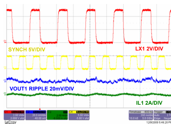
FIGURE 25. STEADY STATE OPERATION CHANNEL 1 AT NO LOAD WITH F_{SW} = 6MHz
