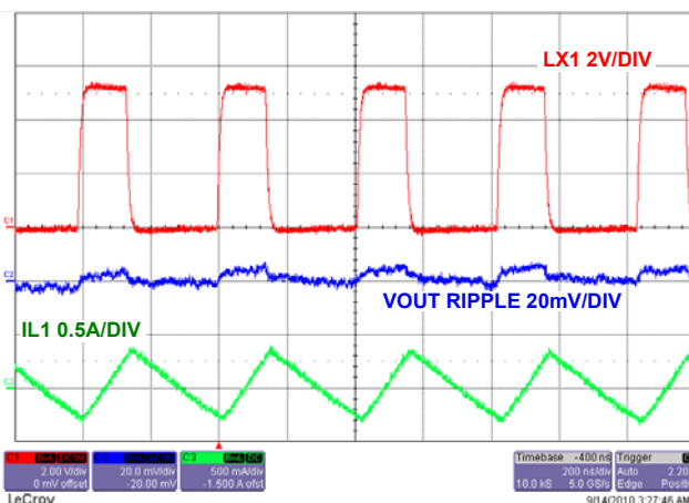
FIGURE 36. STEADY STATE OPERATION AT NO LOAD CHANNEL 1
