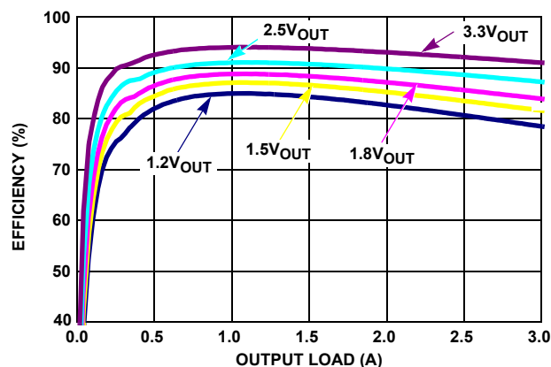
FIGURE 32. EFFICIENCY vs LOAD, 5V IN DUAL CHANNEL 1, T A = +25°C
