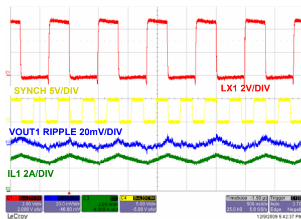
FIGURE 23. STEADY STATE OPERATION CHANNEL 1 AT FULL LOAD WITH F_{SW} = 2.4MHz
