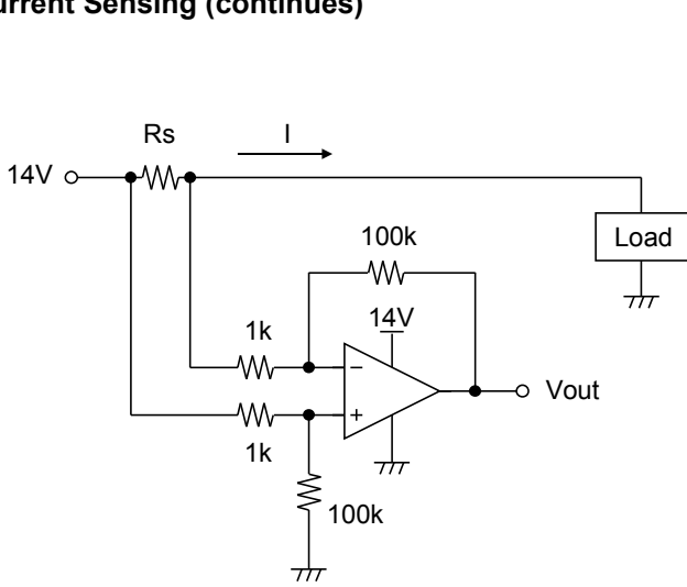
Figure6. High-Side Current Sensing
