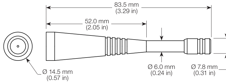
Figure 6. CW LTE Band 5 Antenna Dimensions
