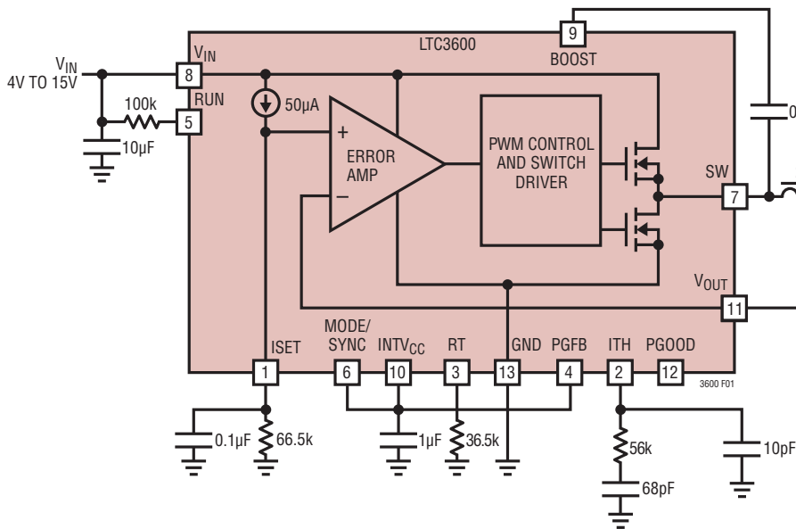
Figure 1. 12V to 3.3V 1MHz Buck Regulator
