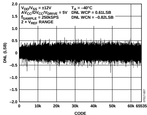
Figure 7. AD7656-1 Typical DNL
