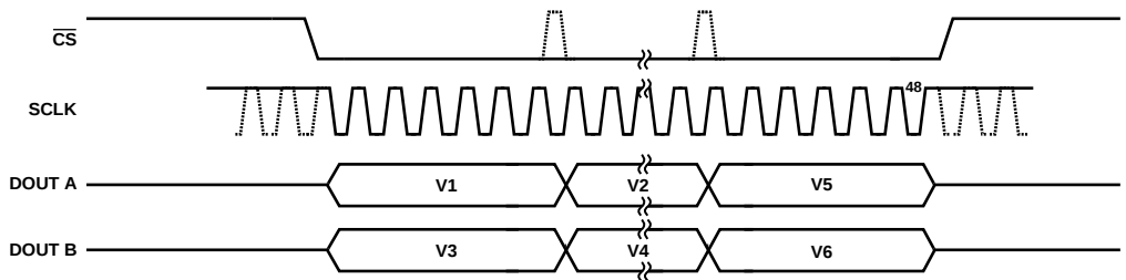
Figure 33. Serial Interface with Two DOUT Lines
