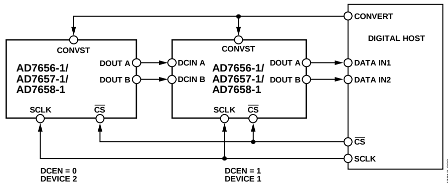
Figure 36. Daisy-Chain Configuration
