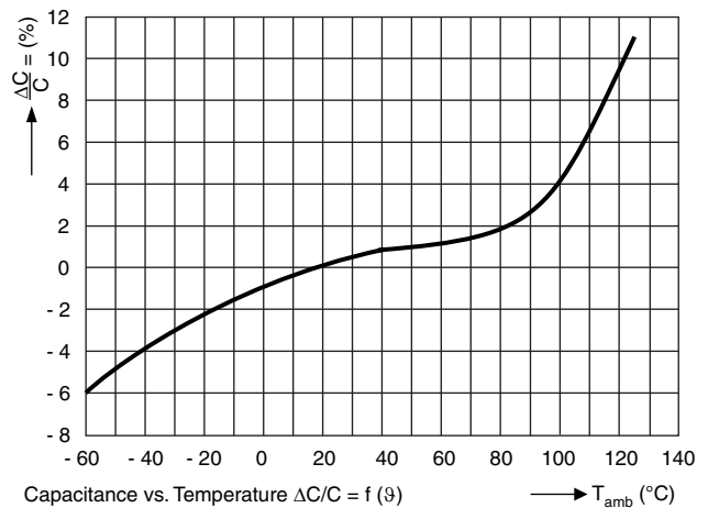
Capacitance vs. Temperature \Delta C/C = f(T) Capacitance as a function of temperature (typical curve)
