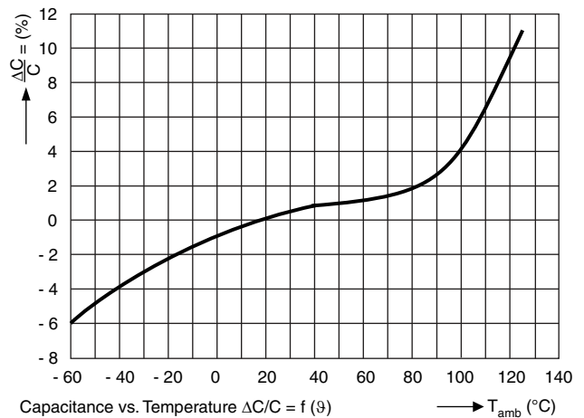
Capacitance vs. Temperature \Delta C/C = f (^\circ\text{C}) Capacitance as a function of temperature (typical curve)
