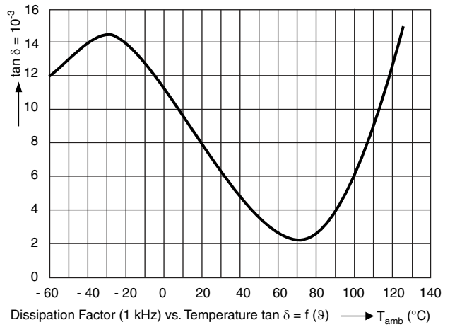
Dissipation Factor (1 kHz) vs. Temperature \tan \delta = f(\vartheta) Dissipation factor as a function of temperature (typical curve)
