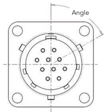
Viewed from receptacle front face. Insulator rotated inside metal body.
