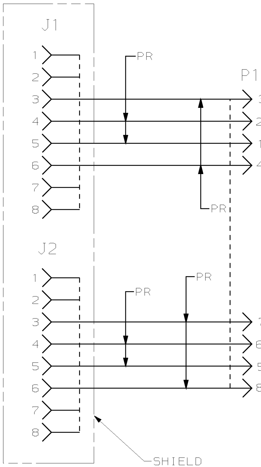
ELECTRICAL SCHEMATIC
