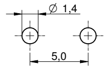
MOUNTING HOLES
