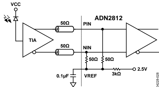
Figure 28. DC-Coupled Application
