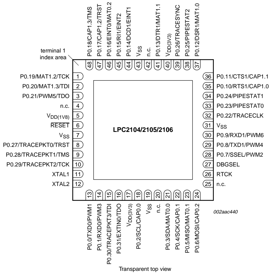
Fig 3. Pin configuration (HVQFN48)
