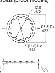
AT508 Lockwasher Steel with Zinc/Chrome (not supplied with splashproof models)
