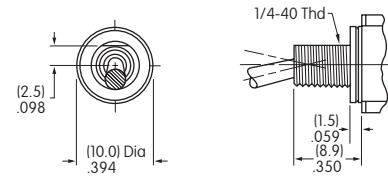
D3 1/4-40 .350" (8.9mm) Threaded Splashproof with D Flat
