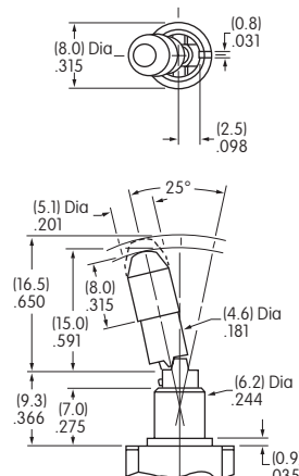
LL2 Smooth with Keyway
