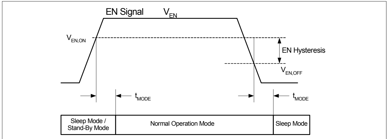
Figure 9 Mode Transition via EN pin
