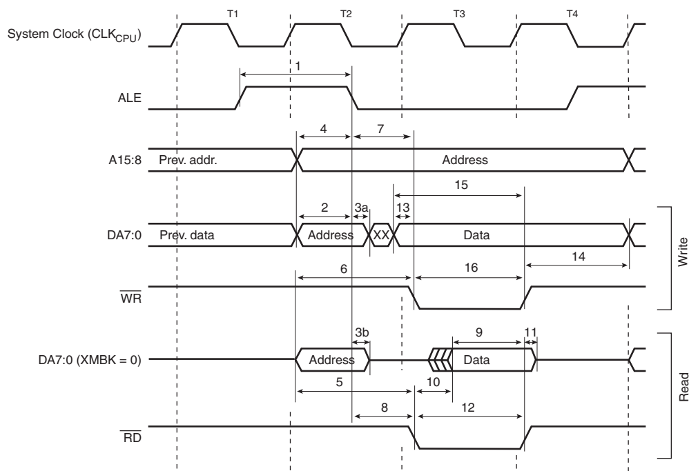
Figure 159. External Memory Timing (SRWn1 = 0, SRWn0 = 0)
