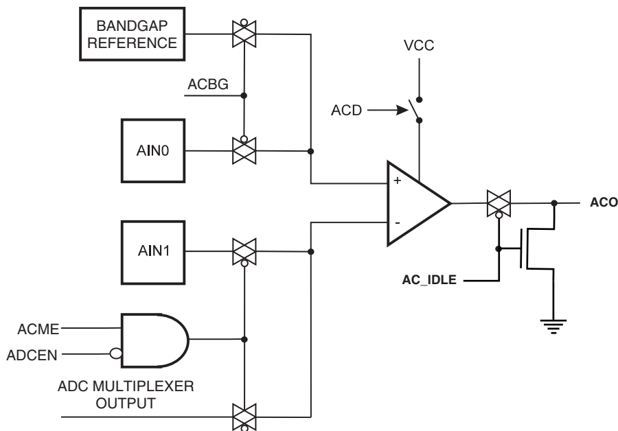
Figure 132. Analog Comparator
