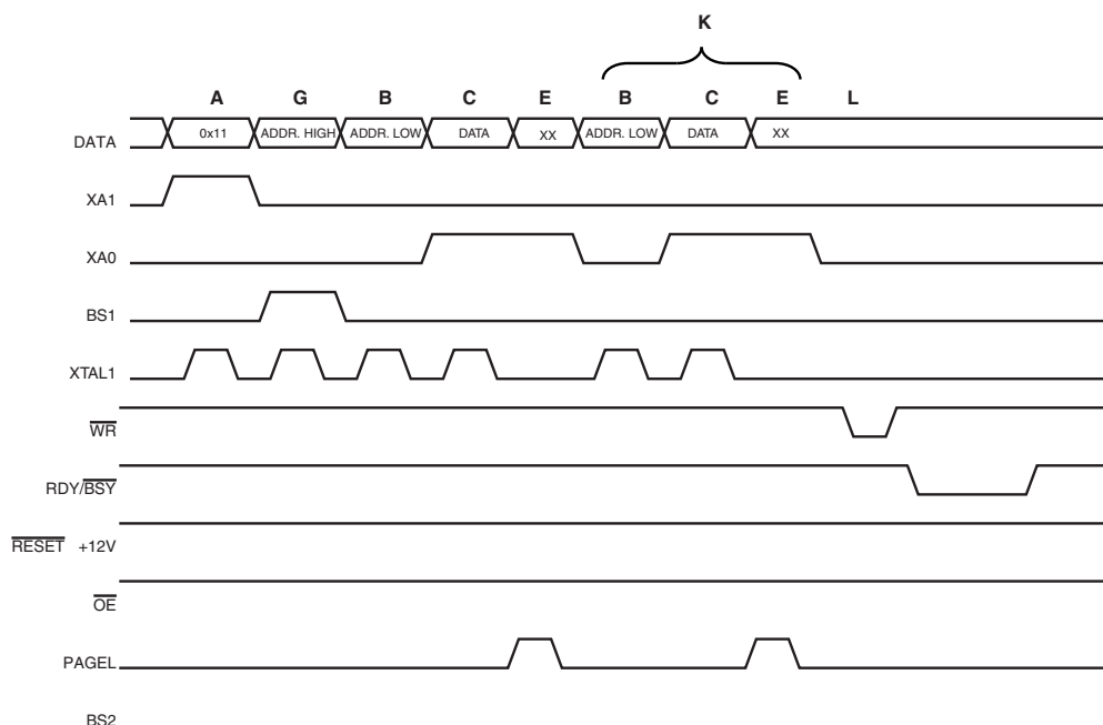
Figure 141. Programming the EEPROM Waveforms
