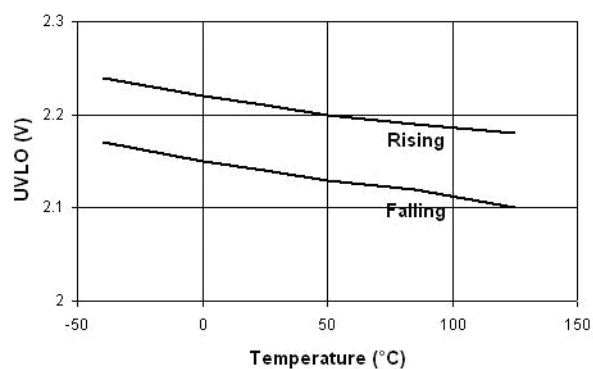
Figure 27. UVLO vs. temperature (STMPS2141/2151)
