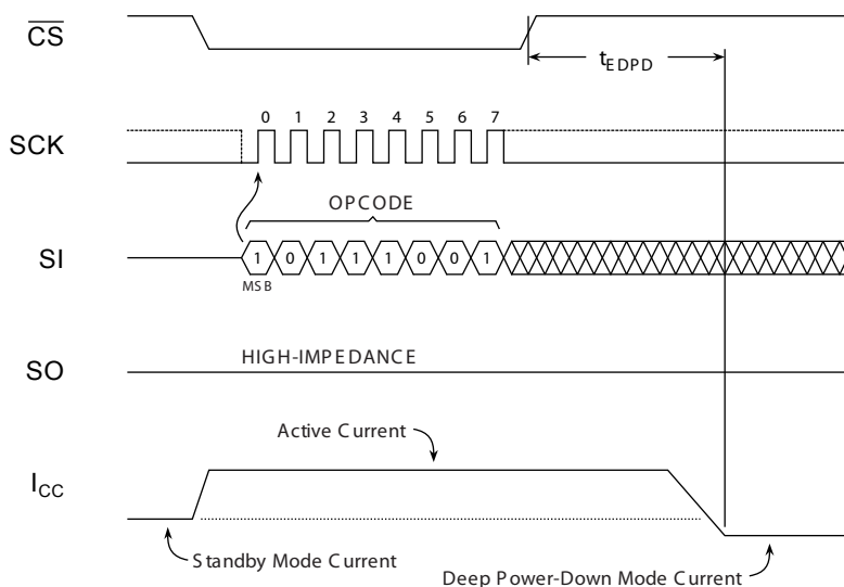
Figure 11-3. Deep Power-Down
