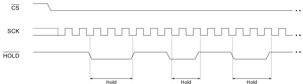
Figure 11-5. Hold Mode
