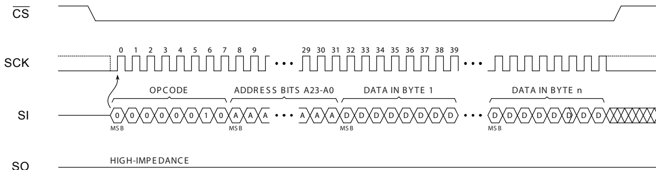
Figure 7-2. Page Program
