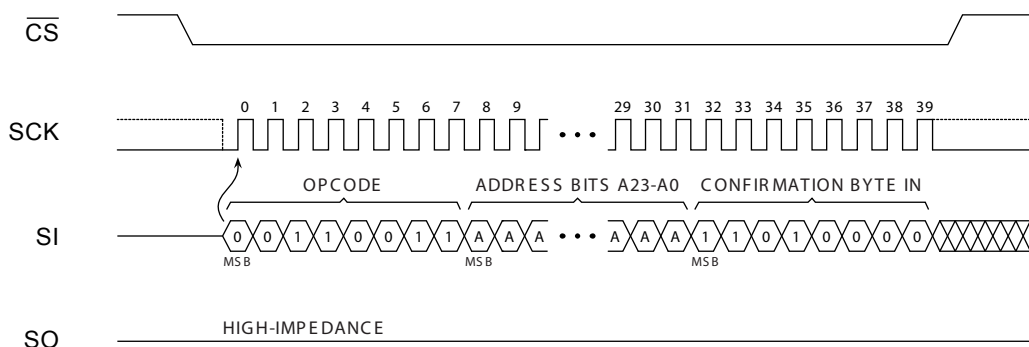
Figure 9-1. Sector Lockdown
