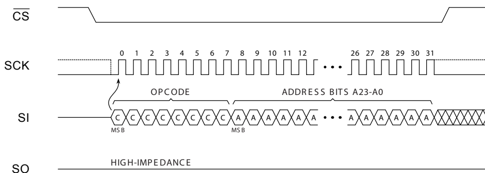
Figure 7-5. Block Erase
