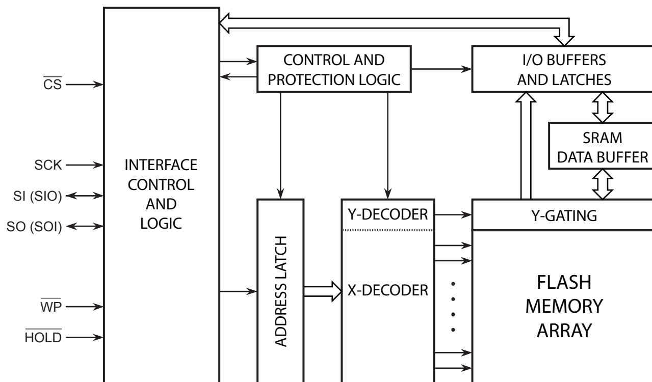
Figure 2-1. Block Diagram
