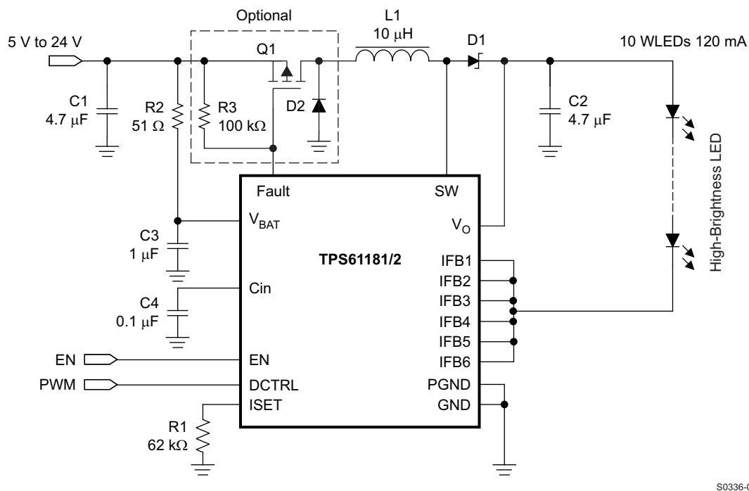
Figure 22. TSP61181/2 for One String High Brightness LEDs Application
