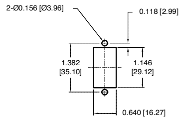
PANEL CUTOUT DETAIL TOLERANCE \pm 0.005 [ \pm 12 ] UNLESS OTHERWISE SPECIFIED
