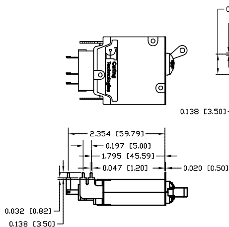
PRINTED CIRCUIT BOARD MOUNTING TERMINAL CODE R
