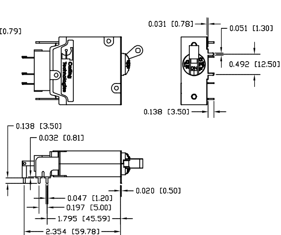
PRINTED CIRCUIT BOARD MOUNTING TERMINAL CODE L
