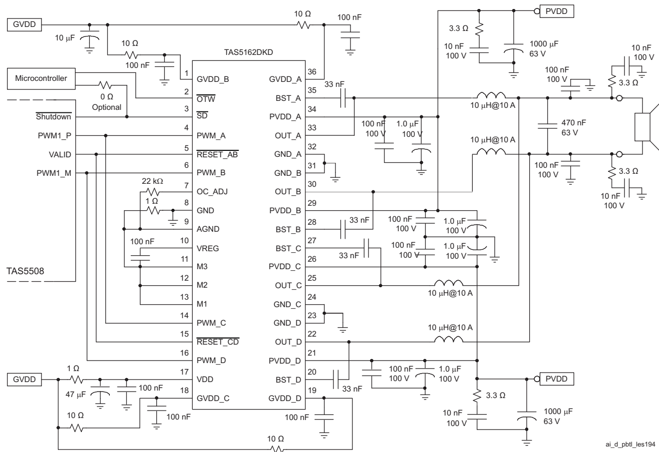
Figure 17. Typical Differential (2N) PBT Application With AD Modulation Filters (For Reference Only, component values and connection will change.)
