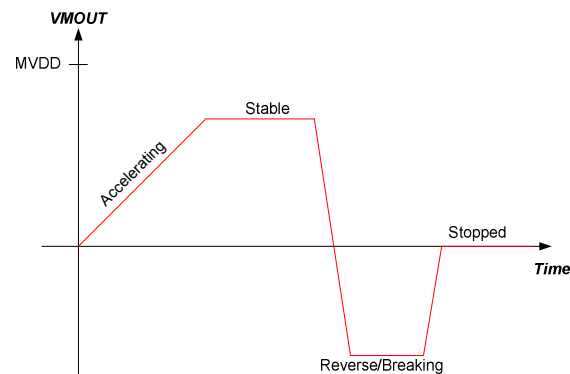
Figure 46 – ERM Drive Signal Example
