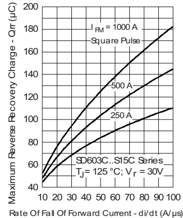
Fig. 16 - Recovery Charge Characteristics
