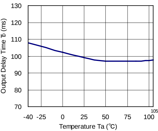
R3116x271A/C
