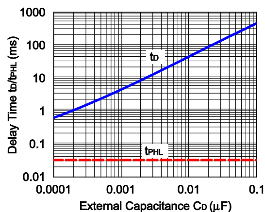
R3116x451A/C
