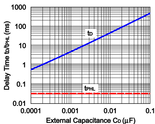
R3116x271A/C
