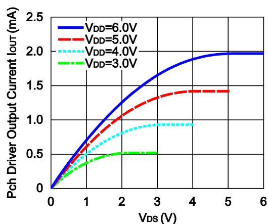
R3116x271C
