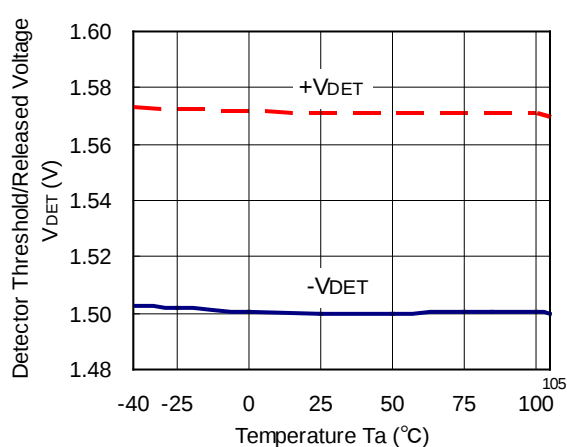
R3116x151A/C
