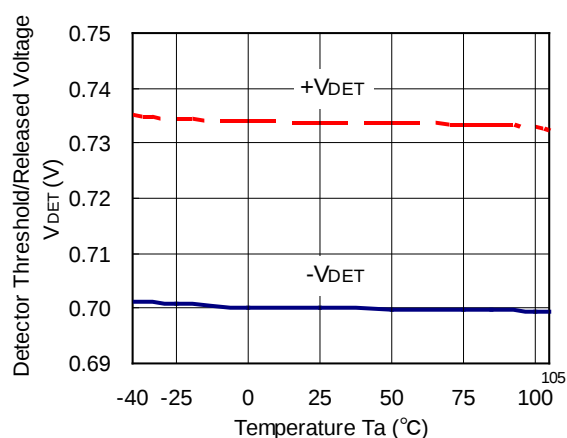
R3116x071A/C
