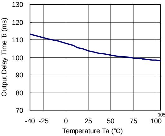
R3116x151A/C
