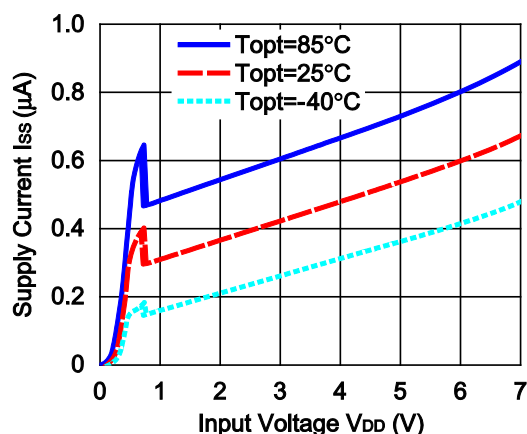
R3116x071A/C
